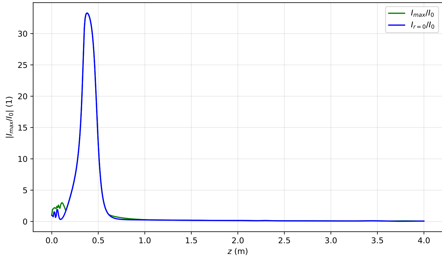
I_{max}(x = 0, y = 0, z)/I_0 , Pin=2.0P_{cr} , artificial time
